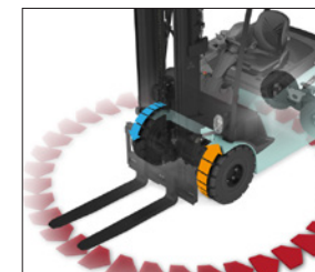
Front wheel dual drive
